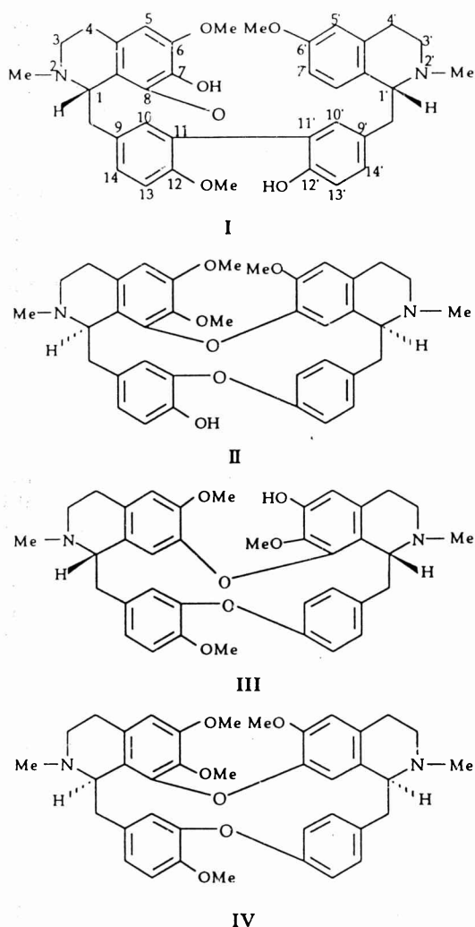
Figure 1. Structures of antioquine (I), berbamine (II), gyrocarpine (III) and isotetrandrine (IV).
